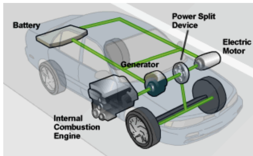
Figure 2. Parts of a hybrid vehicle [4].
